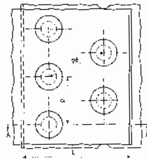
Double-riveted (zigzag) lap joint FIG. 25-8
