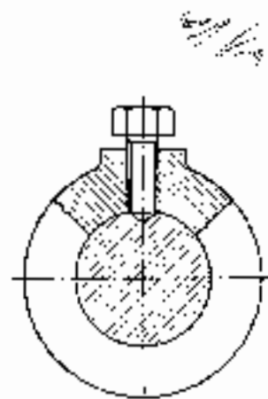
Set-screw
