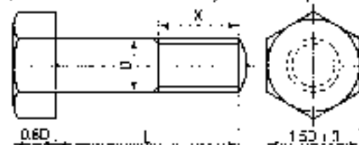
Hexagonal-headed bolt — approximately standard dimensions fig. 24-15
