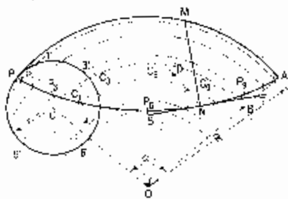
Hypocycloid FIG. 6-35
