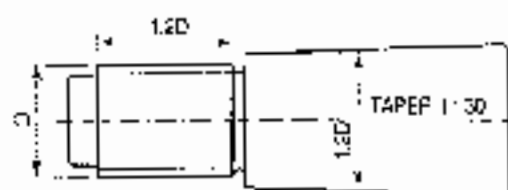
Headless tapered bolt
