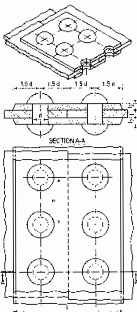
Single-riveted (double straps) butt joint FIG. 25-10
