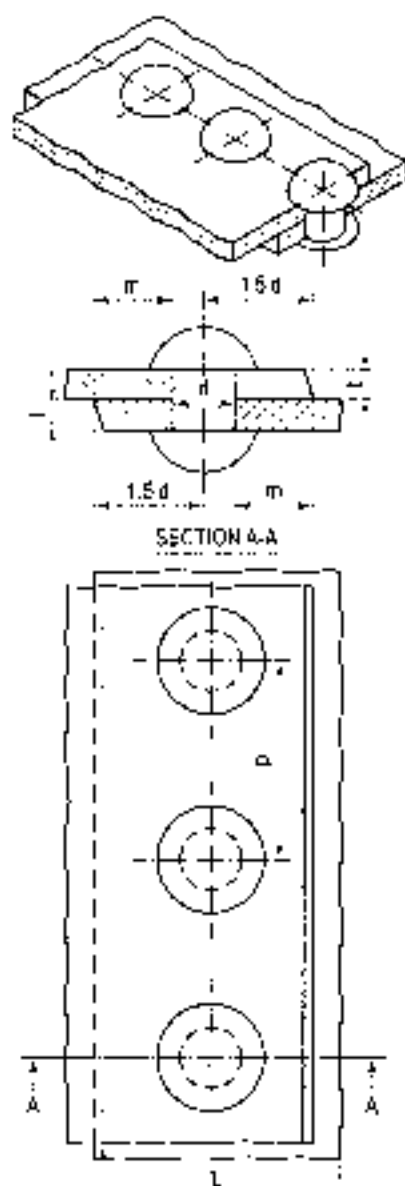
Single-riveted lap joint FIG. 25-6
