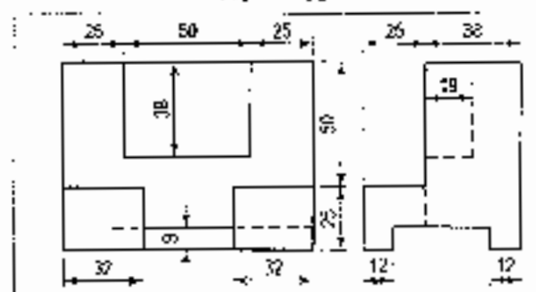
(Third-angle projection)
