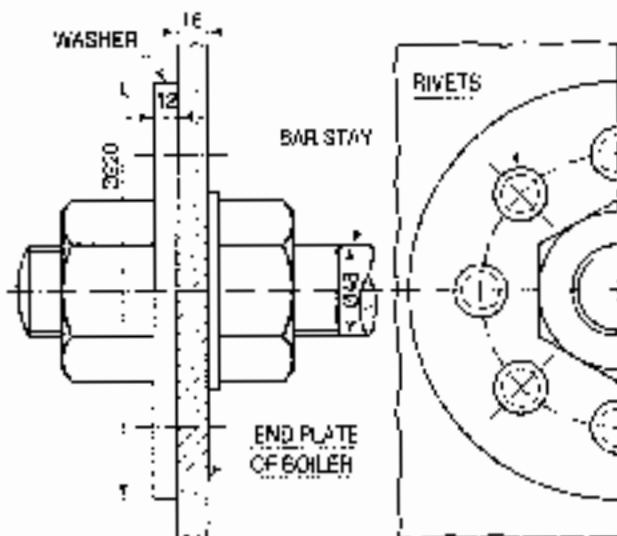
Bar stay
