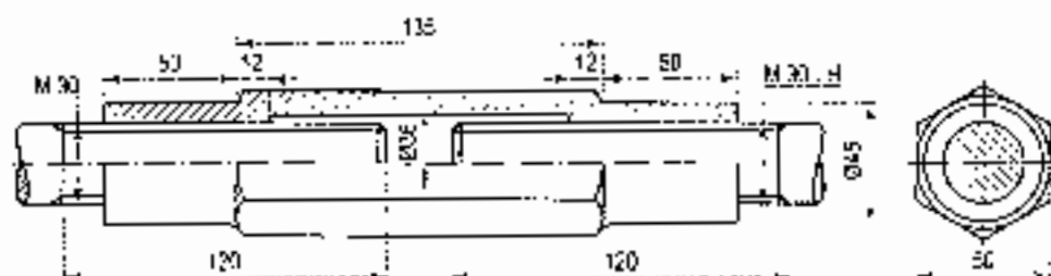
Coupler-nut
