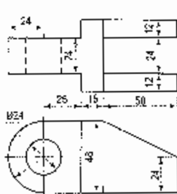
(Third-angle projection)
