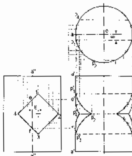
(Third-angle projection)
