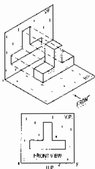
FIRST-ANGLE PROJECTION
