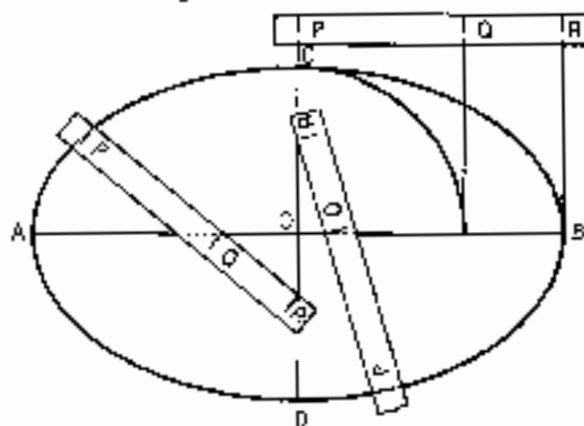
Trammel method
