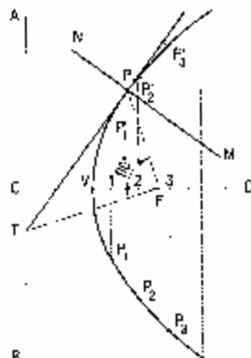
Directrix and focus FIG. 6-14
