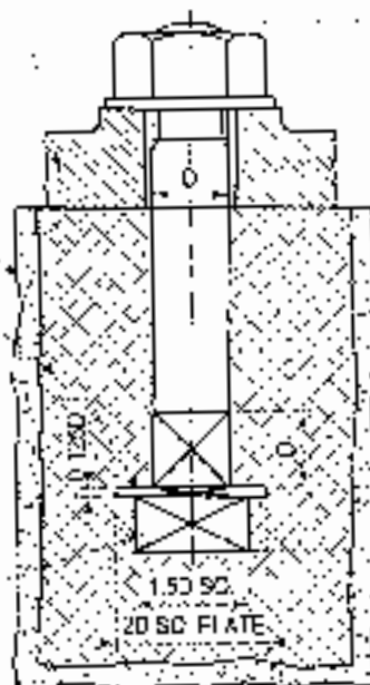
Square-headed bolt FIG. 24-71
