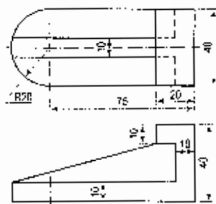
(Third-angle projection)
