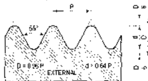
Whitworth thread
