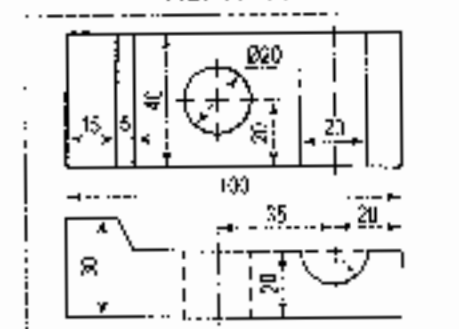
(Third-angle projection)
