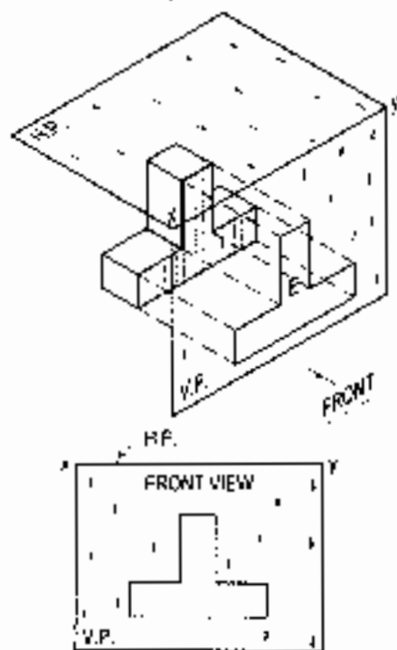
THIRD-ANGLE PROJECTION
