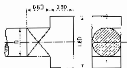
T-headed bolt
