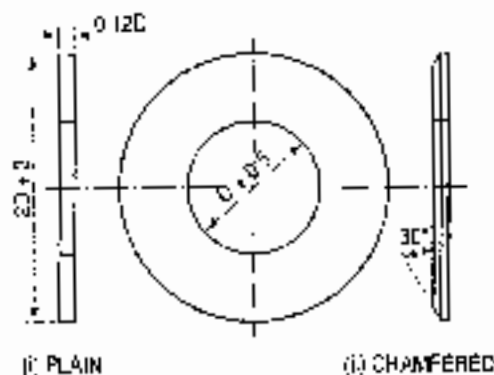
Washers Fig. 24-13
