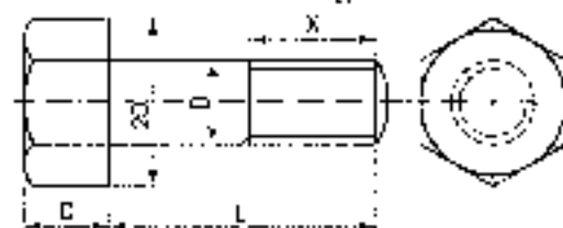
Hexagonal-headed bolt — rough-rule dimensions fig. 24-14
