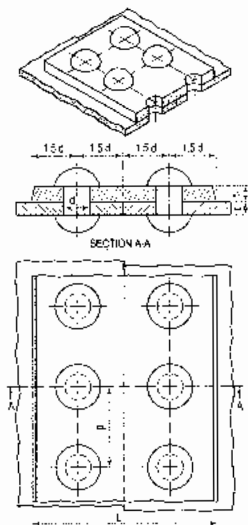
Single-riveted (single strap) butt joint FIG. 25-9
